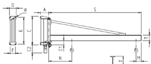
290° Potence murale - Rotation 290°
