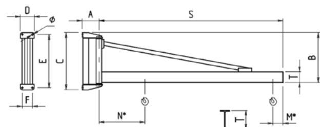
270° Potence murale - Rotation 270°
